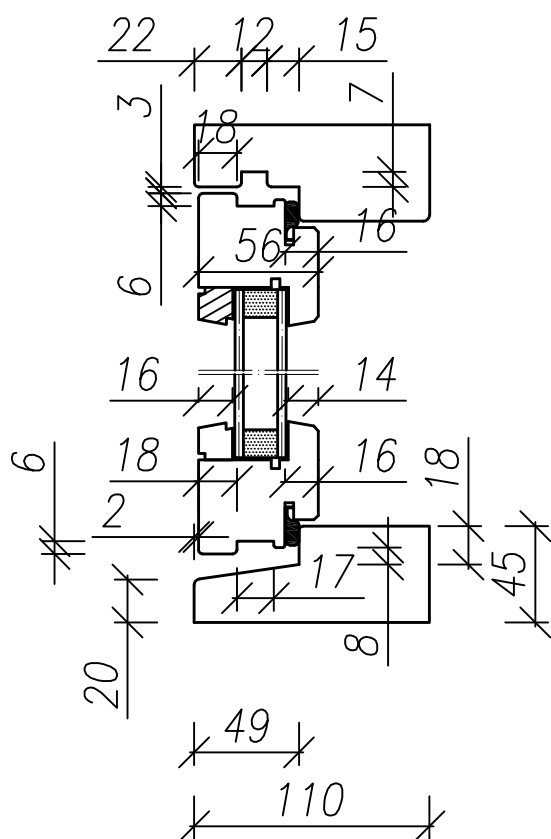
Skandinavian door opening outside vertical section
