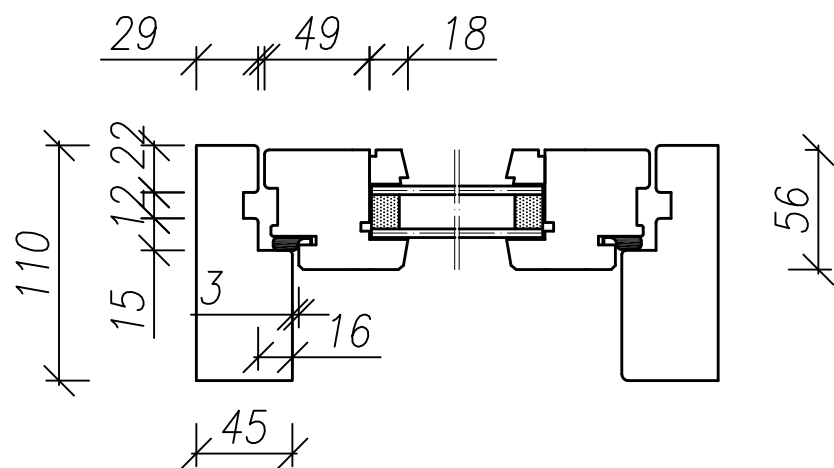
Skandinavian door opening outside horizontal section
