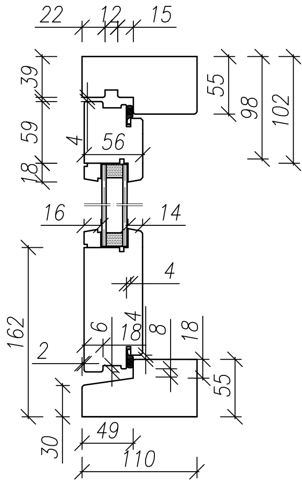
Skandinavian door opening outside vertical section
