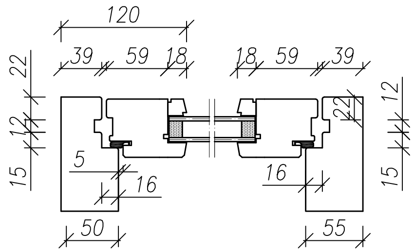
Skandinavian door opening outside horizontal section
