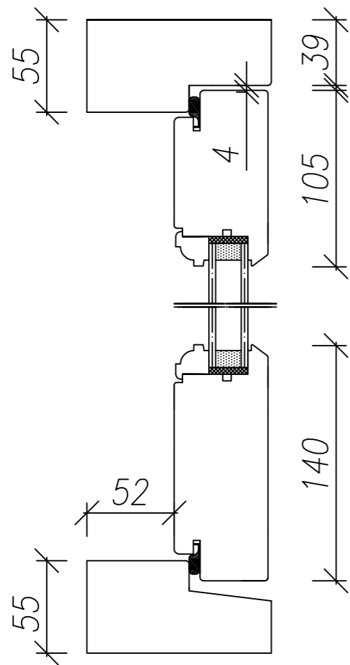
vertical section
