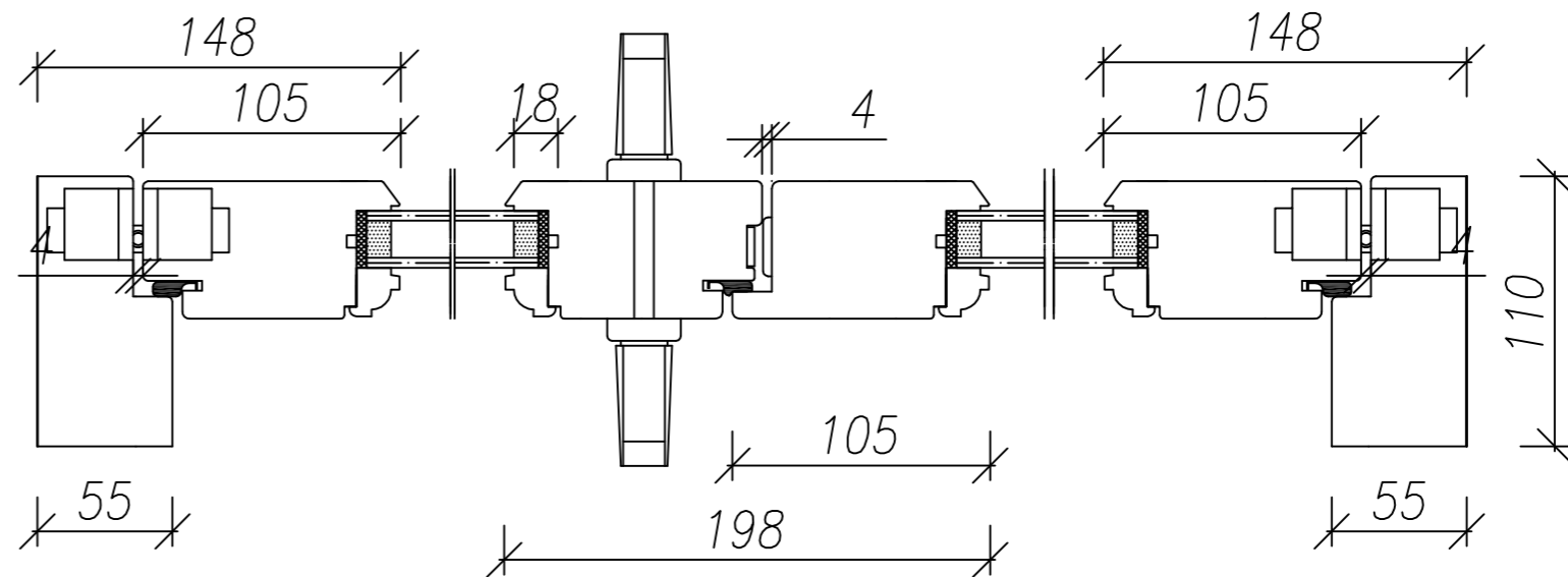
hidden hinges horizontal section
