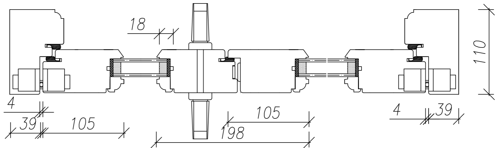
hidden hinges horizontal section
