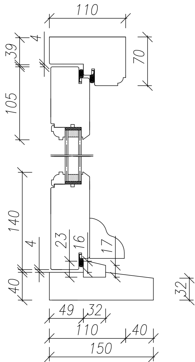
vertical section
