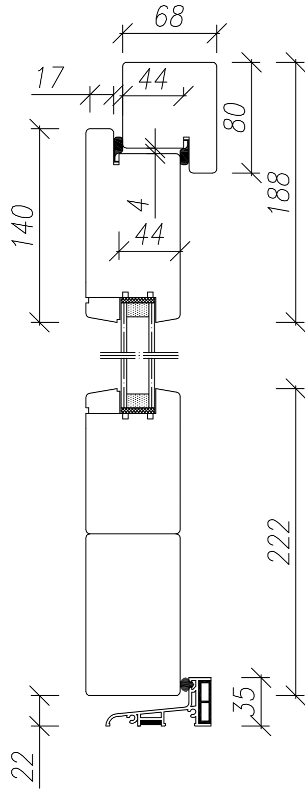
vertical section
