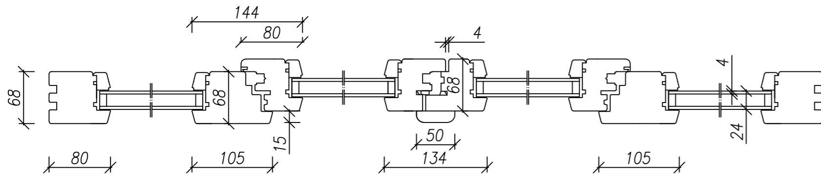
Profile DJ 68 standard
