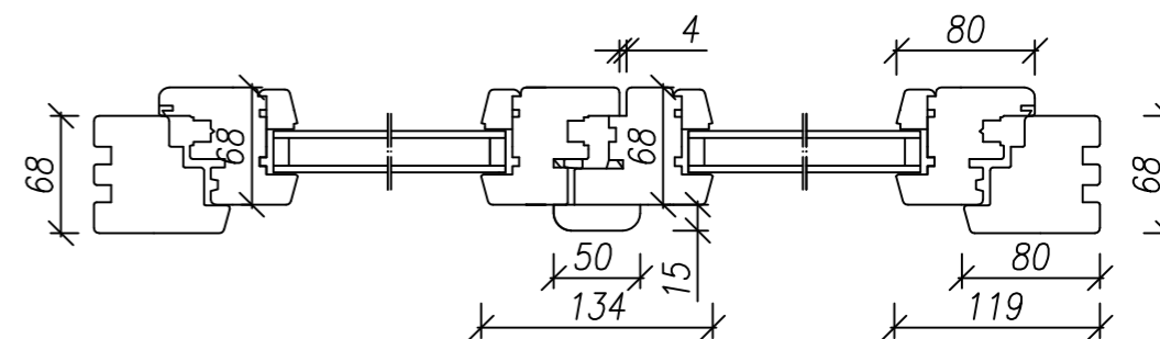
Profile DJ 68 standard - movable column
