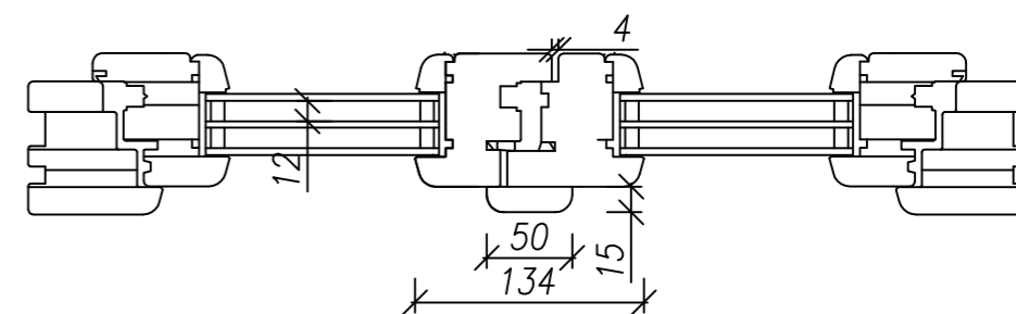
Profile DJ 78 soft line - movable column
