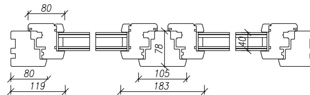
Profile DJ 78 standard - immovable column
