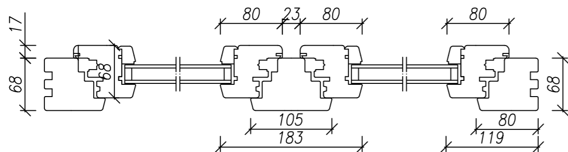
Profile DJ 68 standard - immovable column
