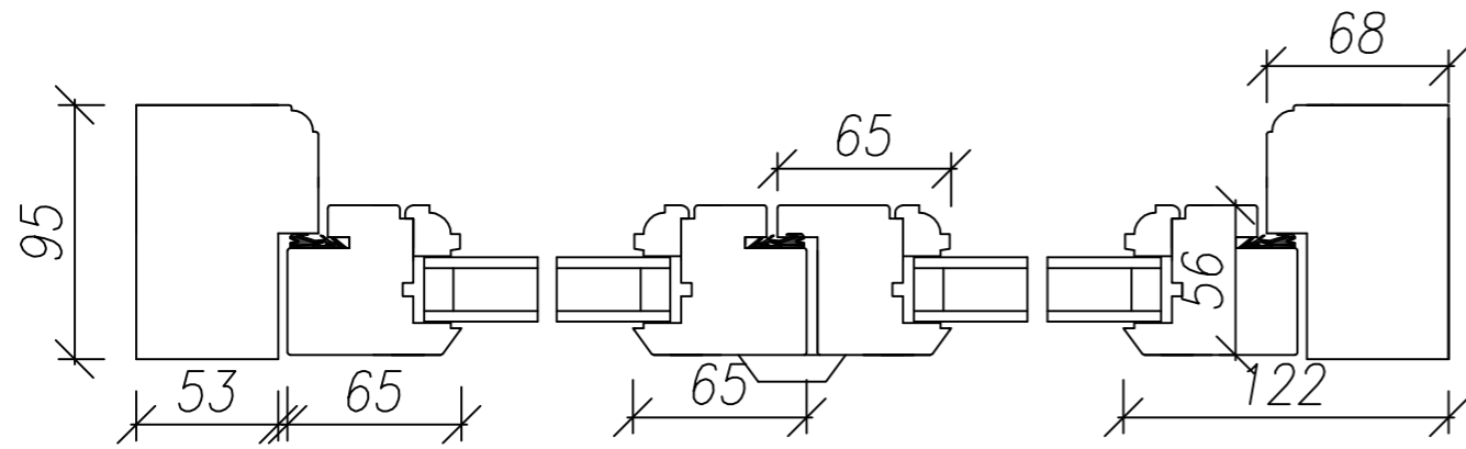
movable column - horizontal section
