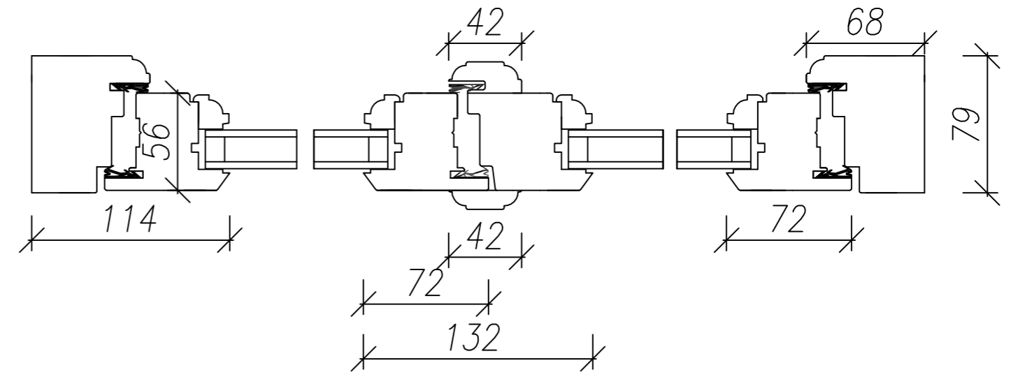
movable column - horizontal section
