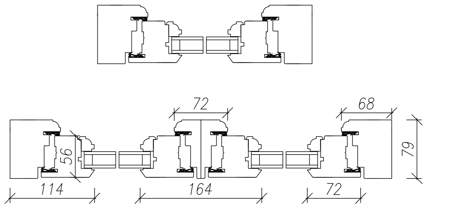
horizontal section
