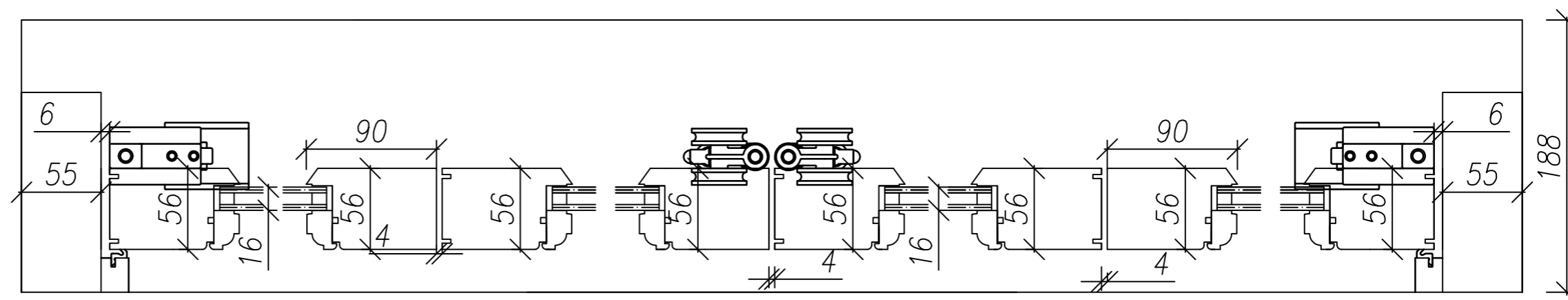
horizontal section
