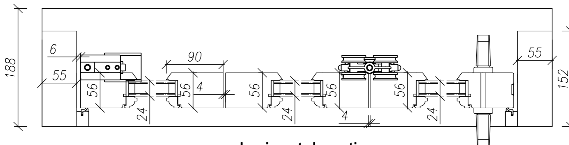
horizontal section
