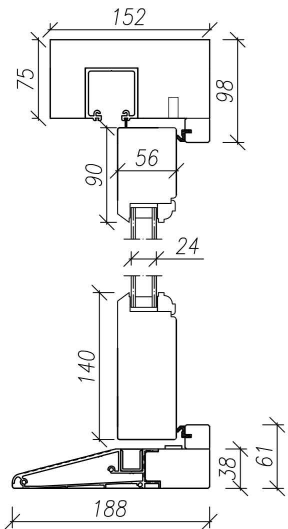
vertical section
